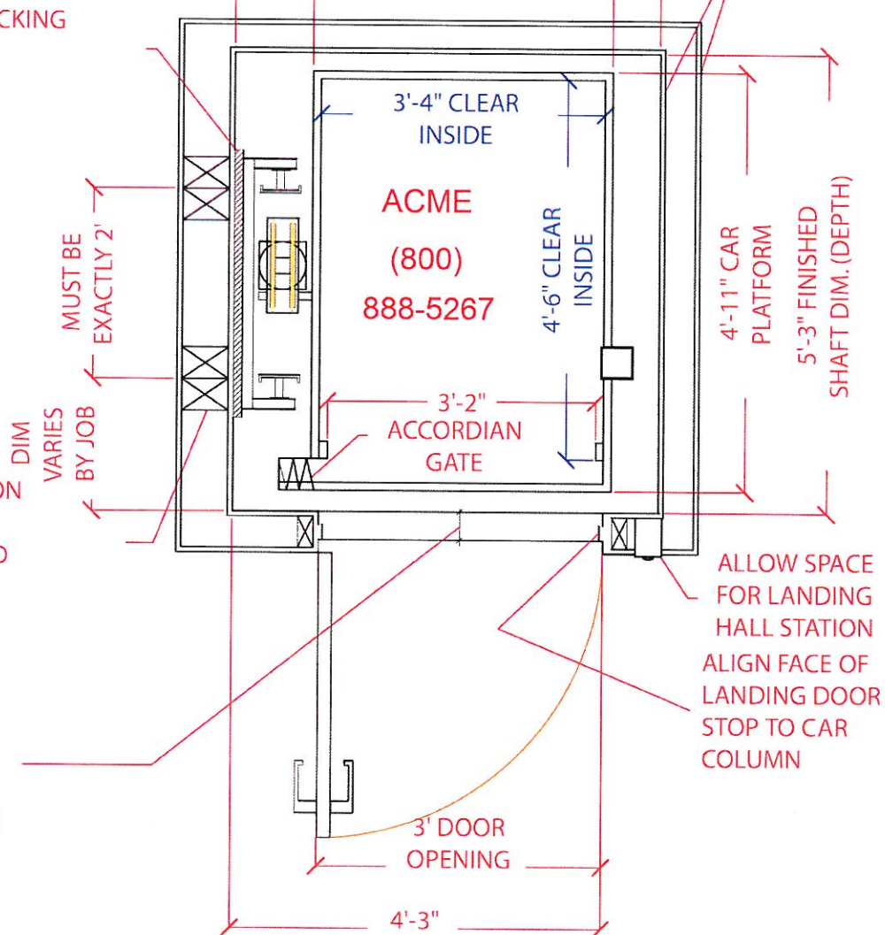
TYPICAL HOME ELEVATOR FLOOR PLAN
