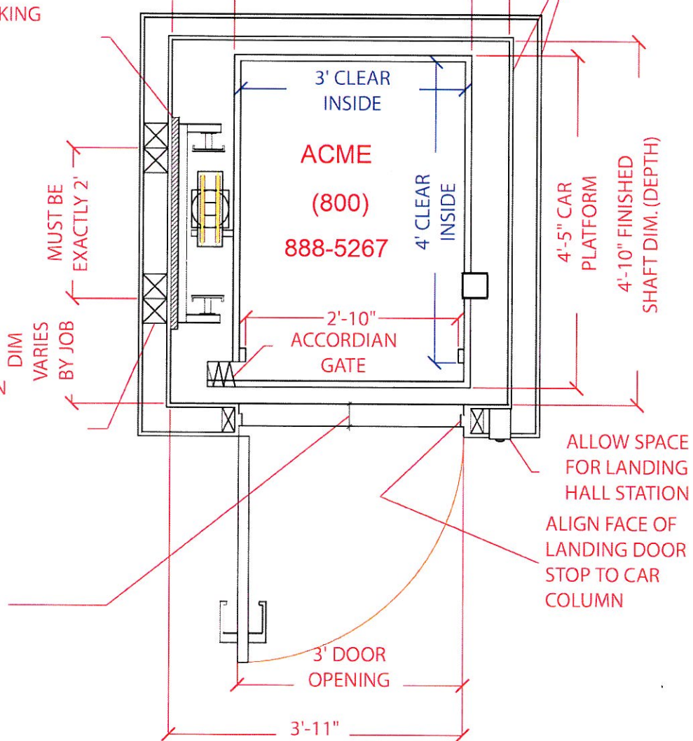
TYPICAL HOME ELEVATOR FLOOR PLAN
